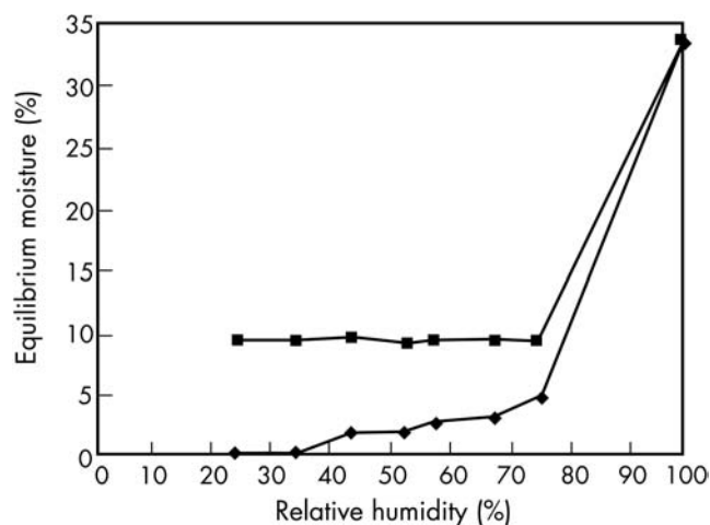
Figure 1: Sorption-desorption isotherm for anhydrous dextrose granules.
