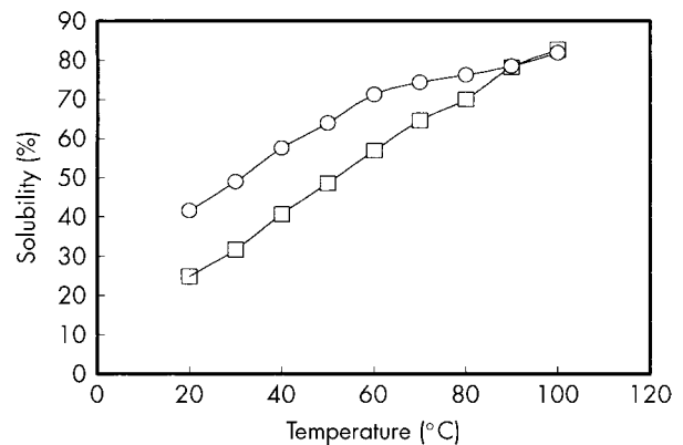
Figure 3: Solubility of isomalt types in water. (2) □: GalenIQ 720 (Palatinit GmbH) ○: GalenIQ 721 (Palatinit GmbH)
