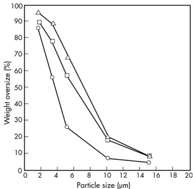
Figure 2: Particle-size distribution of calcium carbonate (Sturcal, Rhodia).
