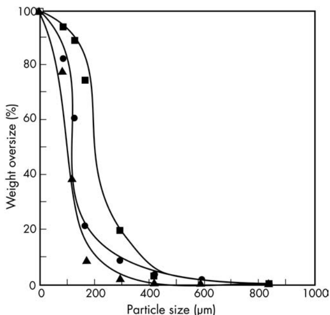
Figure 3: Particle size distribution of granulated xylitol ( Xylitab , Danisco Sweeteners Ltd.).
