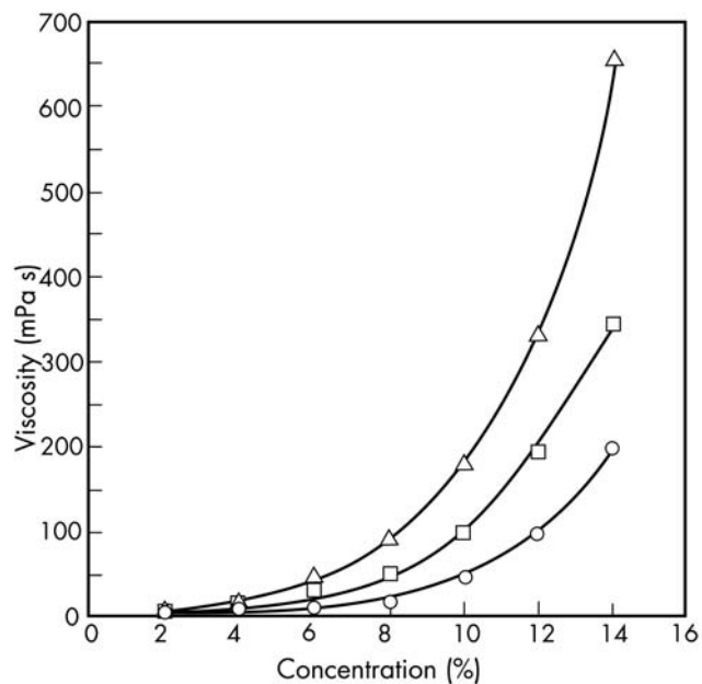
Figure 3: Dynamic viscosity of hypromellose phthalate (HP-50) (Shin-Etsu Chemical Co. Ltd.) in various solvent mixtures at 20°C. (11) ○: Acetone : ethanol (1 : 1) □: Dichloromethane : ethanol (1 : 1) △: Ethanol : water (1 : 1)
