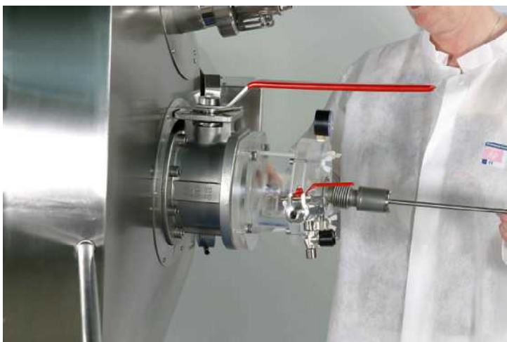
Lock for taking out samplings during process
