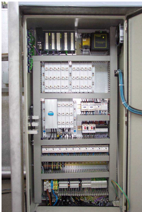
Switch box with S7-300
