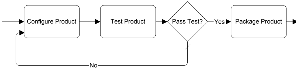
Figure 84 An Until Loop
